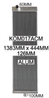
KOMATSU DUMP TRUCK HD785 Left Module
